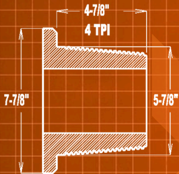
6-5/8" REG API PIN
