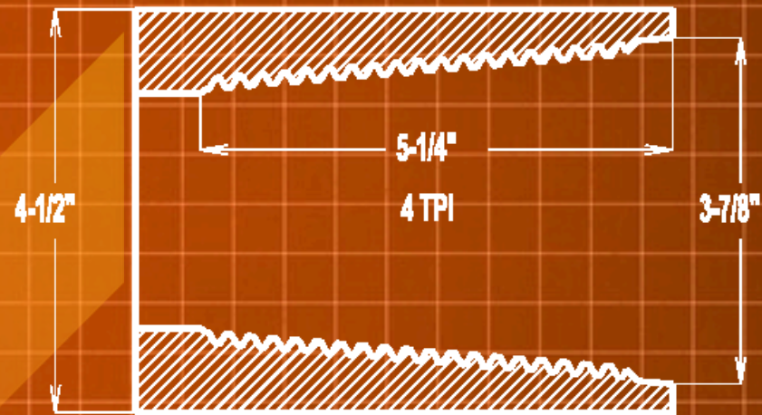
3.44-4 BOX
