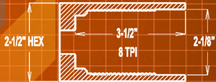
2-1/8" LP BOX
