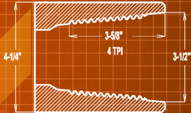
2-7/8" I F BOX
