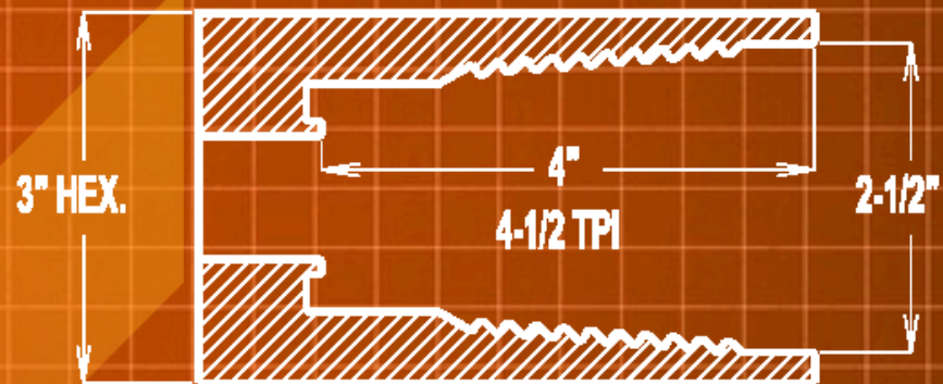
2-1/2" RAMON BOX
