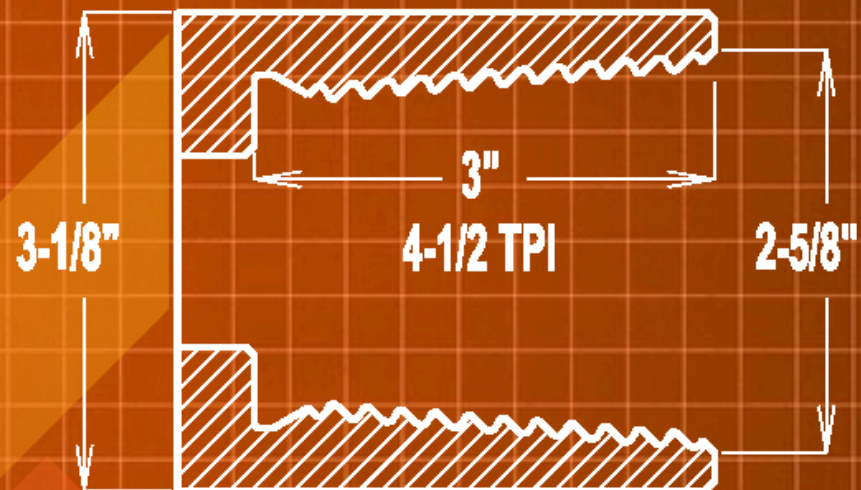
2-5/8" FS1 BOX #700
