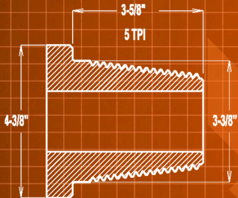
3-1/2" REG API PIN
