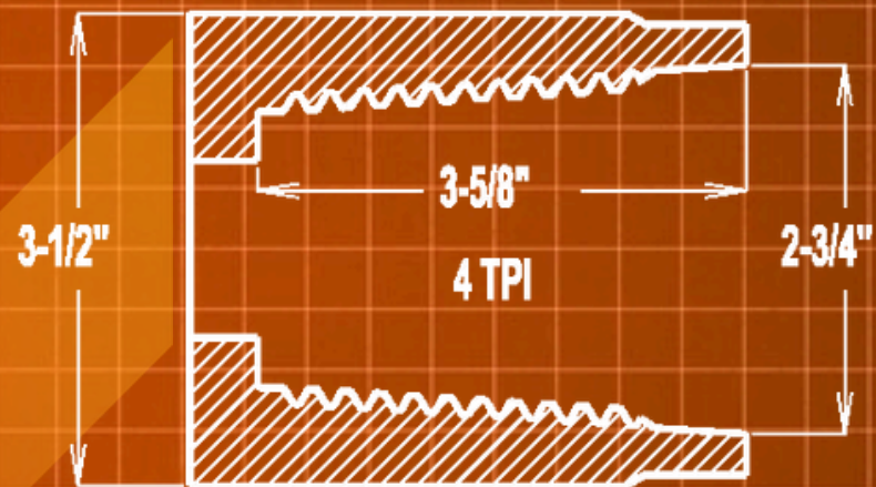
2.59-4 BOX
