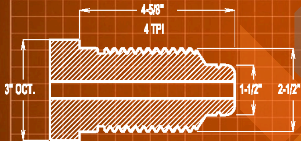
2-1/2" CASE BSW PIN
