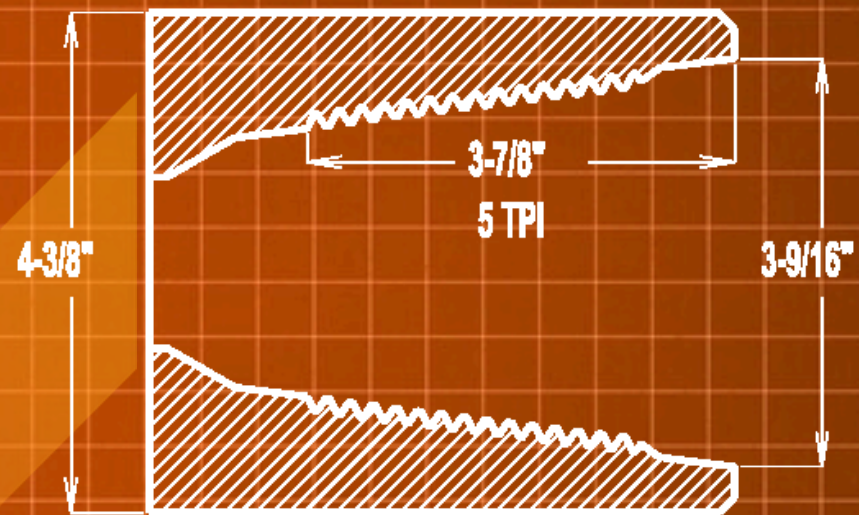
3-1/2" REG API BOX
