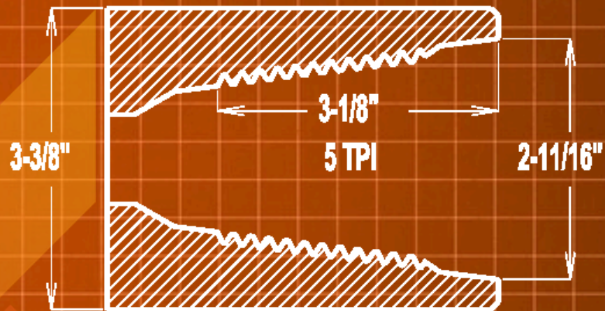
2-3/8" REG API BOX
