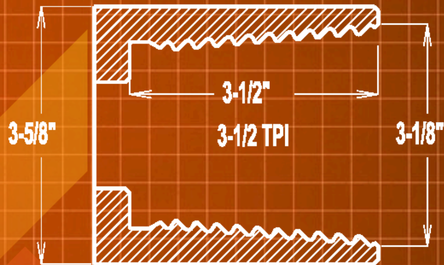
3-1/2" FS1 BOX #800
