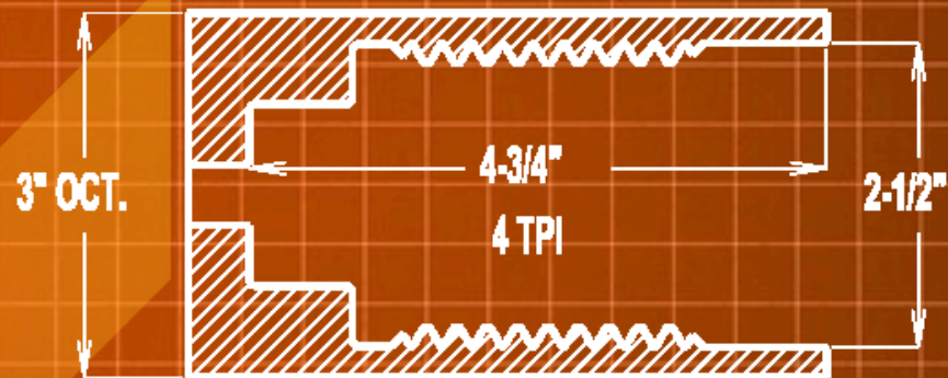
2-1/2" CASE BSW BOX
