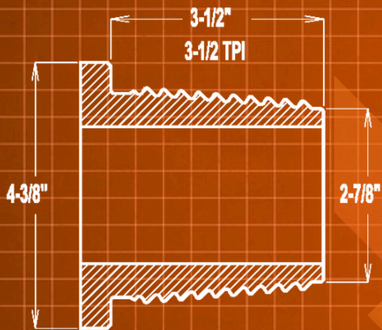
3-1/2" FS1 PIN #1000
