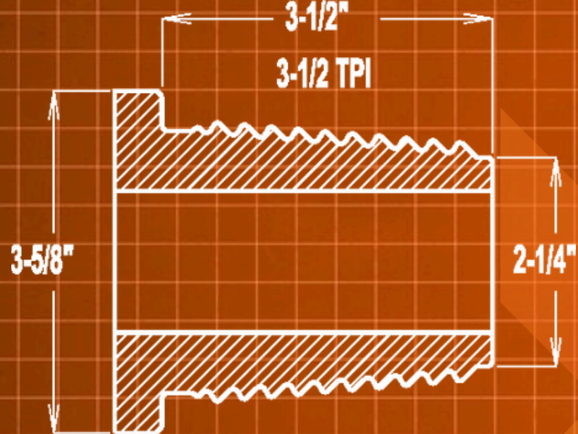
3-1/2" FS1 PIN #800
