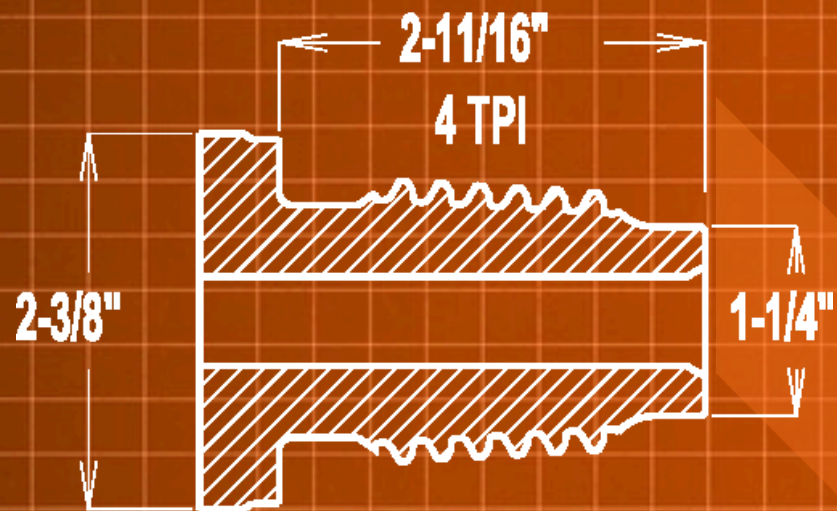
1.47-4 PIN
