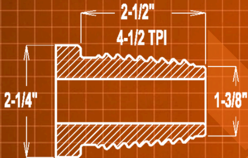
2.06" FS1 PIN #400
