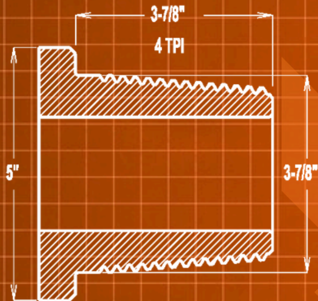
3-1/2" I F PIN
