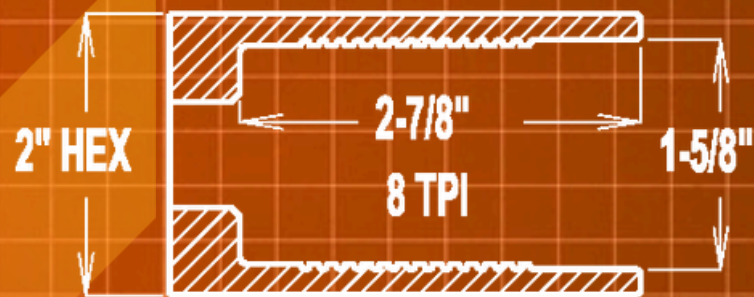
1-5/8" LP BOX
