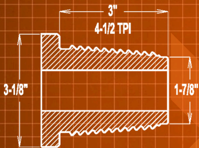
2-5/8" FS1 PIN #700
