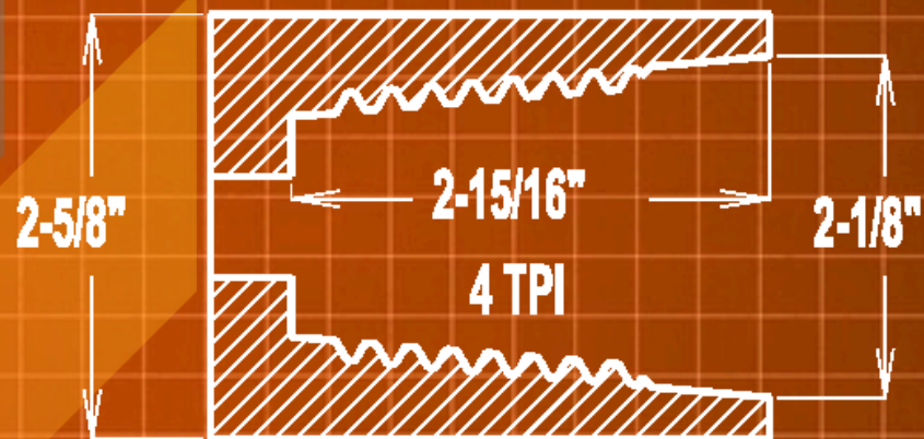
1.94-4 BOX
