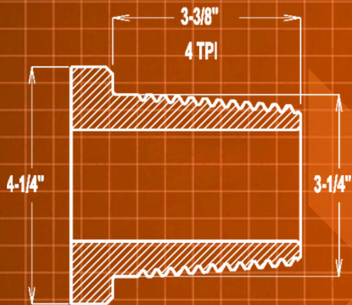
2-7/8" I F PIN
