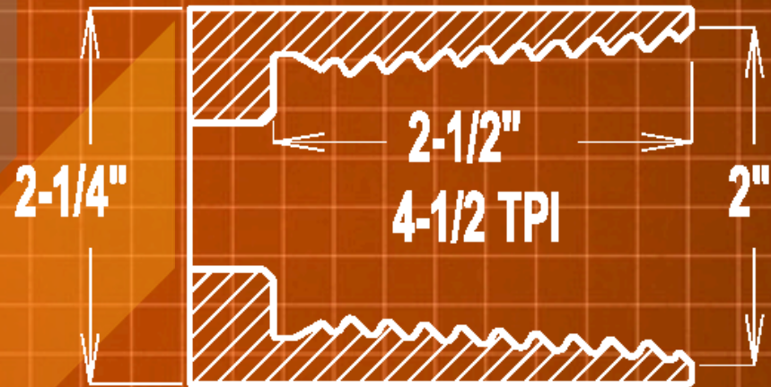
2.06" FS1 BOX #400
