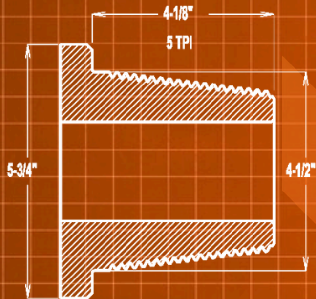
4-1/2" REG API PIN
