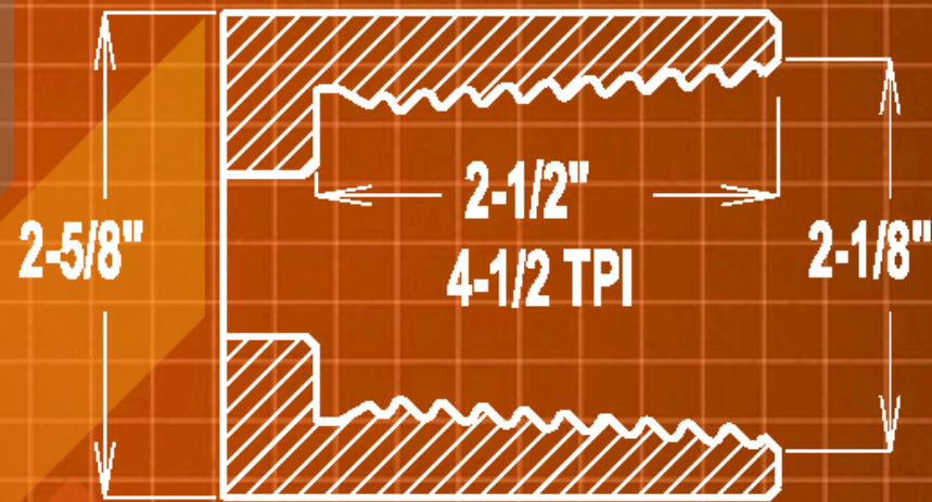
2-3/8" FS1 BOX #600
