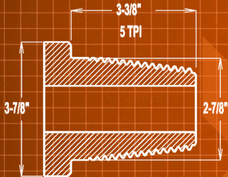
2-7/8" REG API PIN
