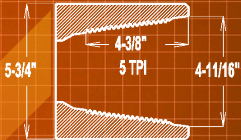
4-1/2" REG API BOX
