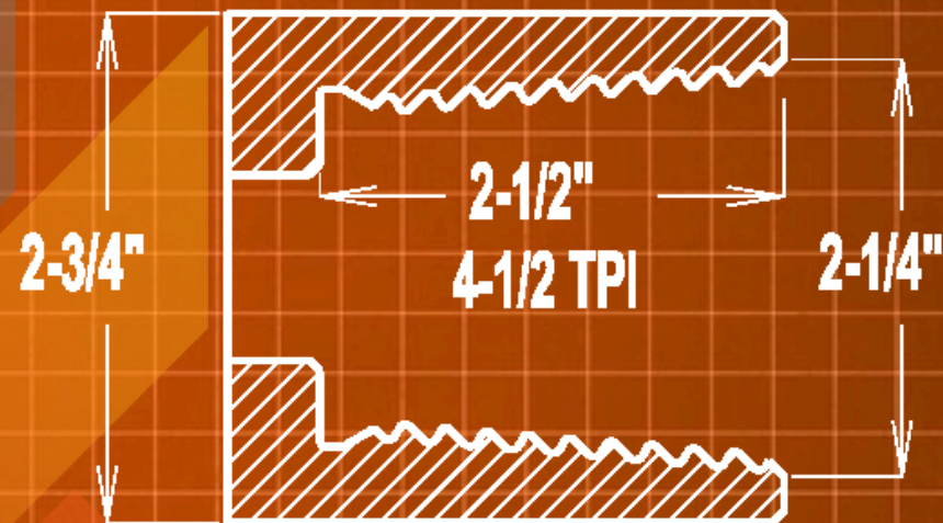
2-3/8" FS1 BOX #650
