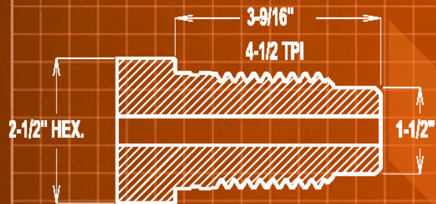
2" UNJ PIN
