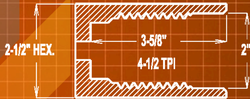
2" UNJ BOX
