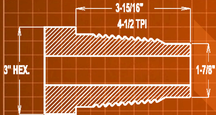
2-1/2" RAMON PIN
