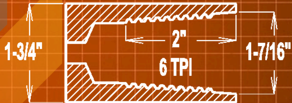
1.41-6 BOX
