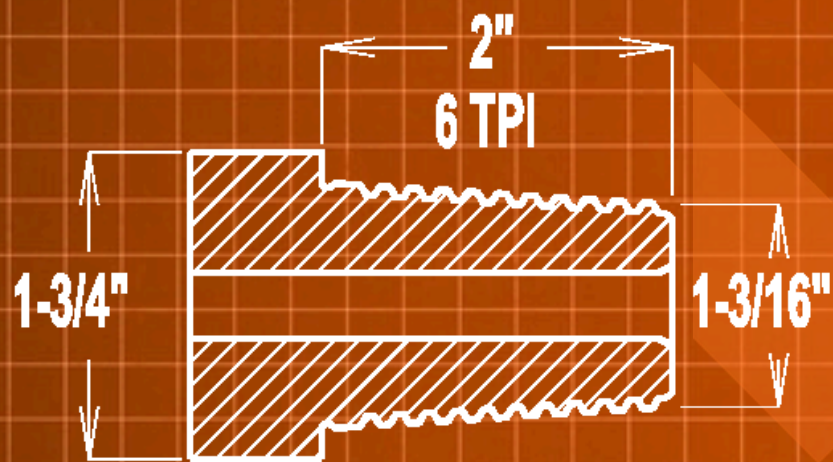
1.41-6 PIN
