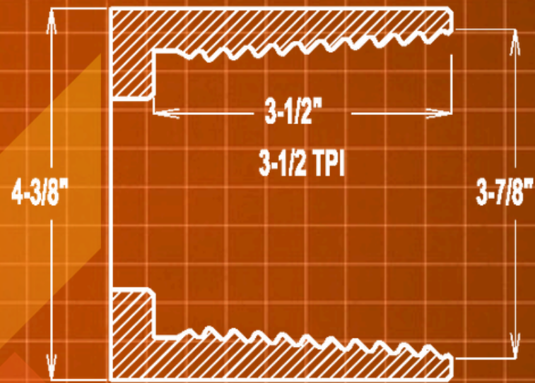
3-1/2" FS1 BOX #1000
