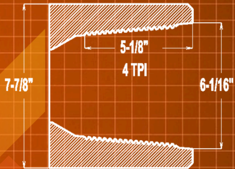
6-5/8" REG API BOX
