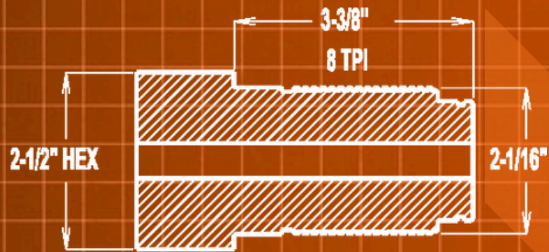
2-1/8" LP PIN
