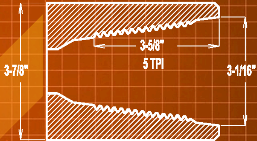
2-7/8" REG API BOX
