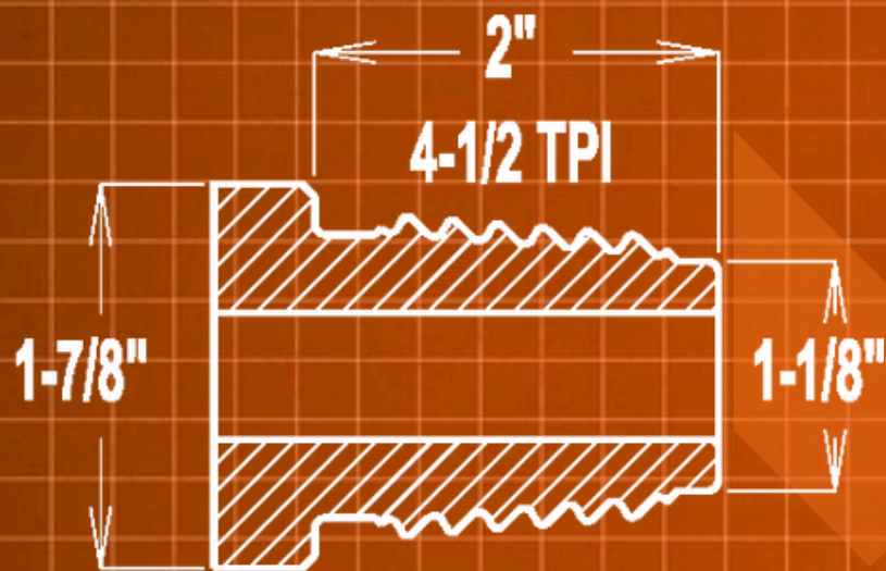
1.66" FS1 PIN #200
