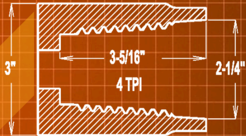
2.11-4 BOX
